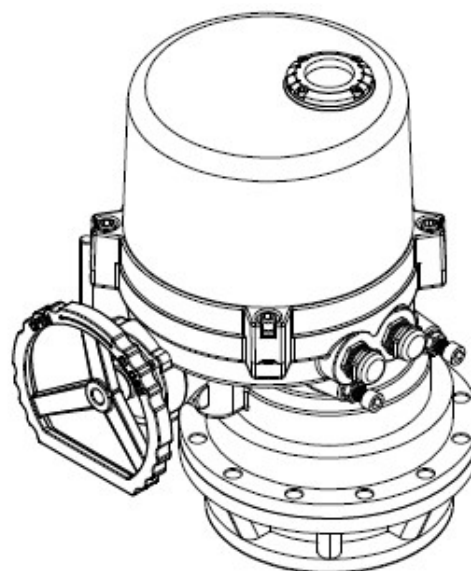
Actuator type CAR-H S200 - 250
