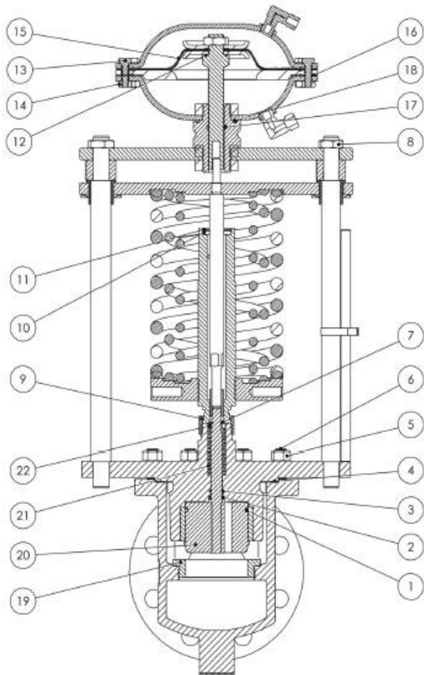
VALVE TD-56-2 DN15-80 PN16/25
